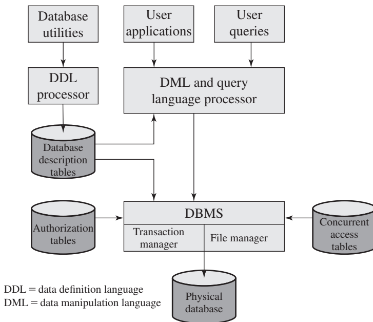
Figure 5.1 DBMS Architecture
