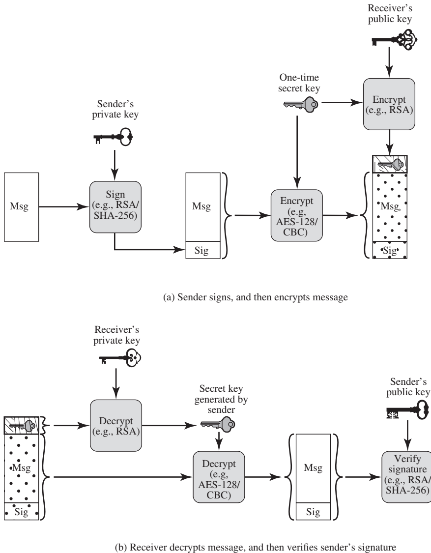
Figure 22.1 Simplified S/MIME Functional Flow
