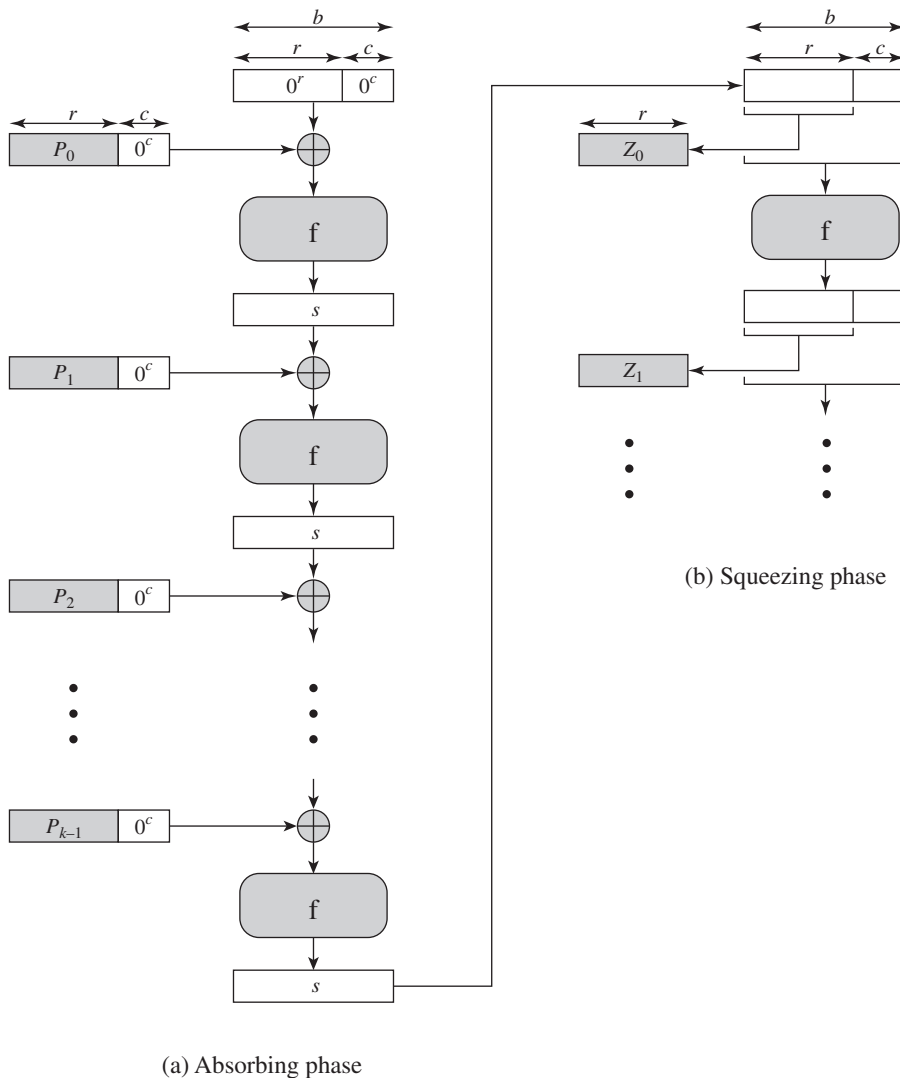
Figure J.2 Sponge Construction
