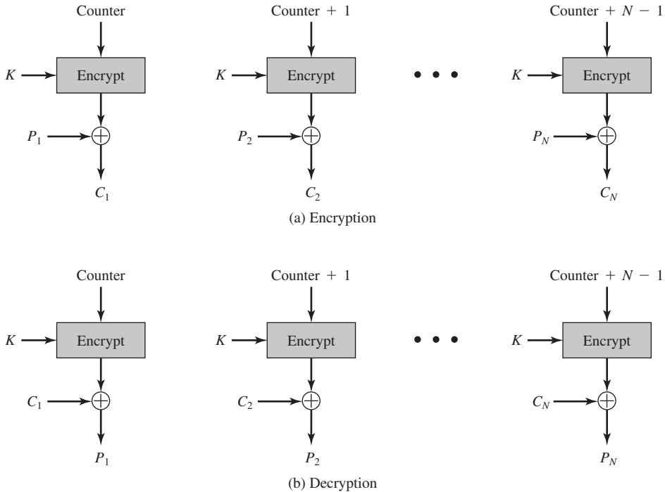
Figure 20.9 Counter (CTR) Mode
