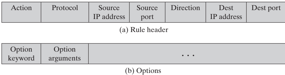
Figure 8.10 Snort Rule Formats
