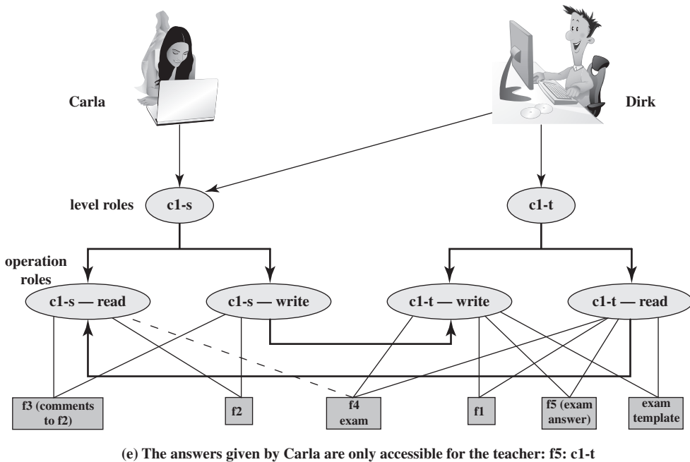
Figure 27.2 Example of Use of BLP Concepts
