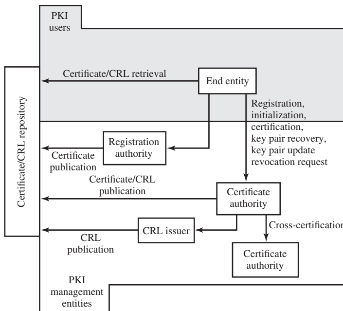
Figure 23.4 PKIX Architectural Model
