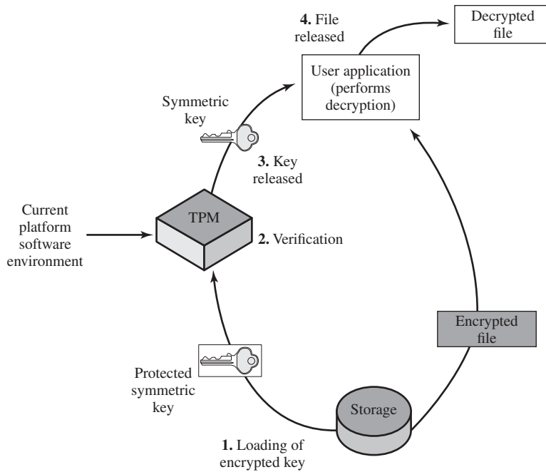
Figure 27.12 Decrypting a File Using a Protected Key
