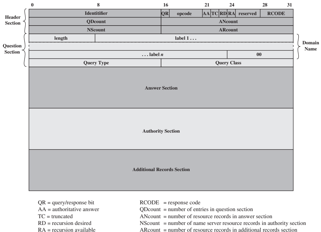
Figure H.5 DNS Message Format
