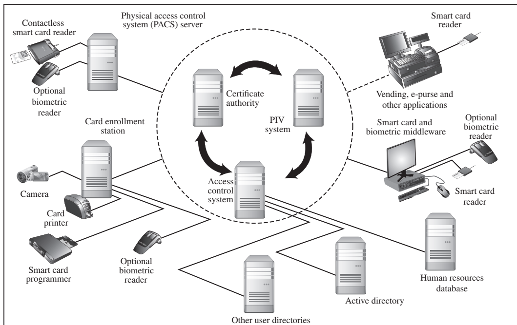
Figure 16.3 Convergence Example
