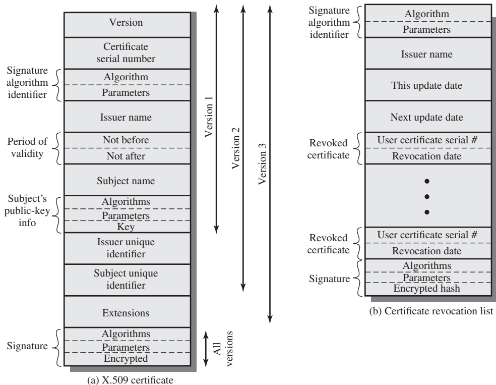
Figure 23.3 X.509 Formats
