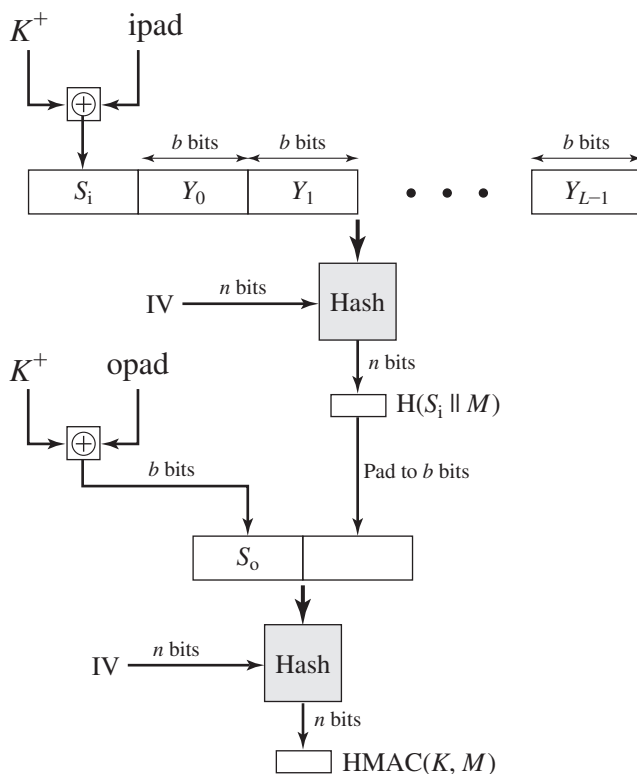
Figure 21.4 HMAC Structure
