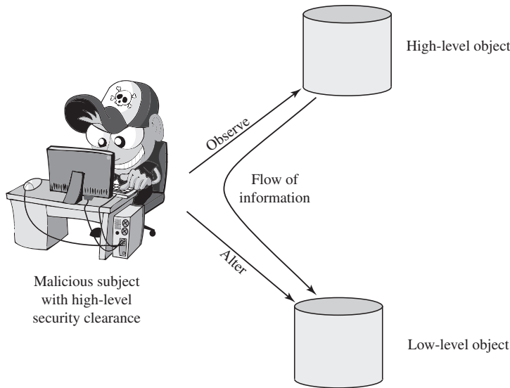
Figure 27.1 Information Flow Showing the Need for the *-Property
