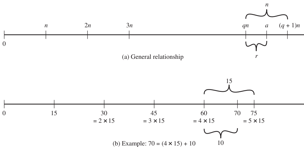
Figure B.1 The Relationship a = qn + r ; 0 < r < n
