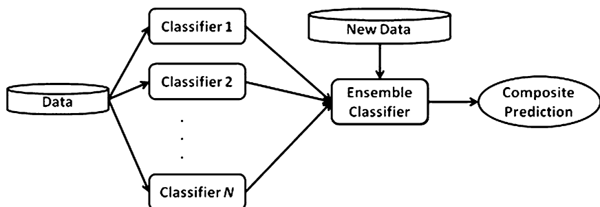
Figure 14.1 Ensemble Classification
