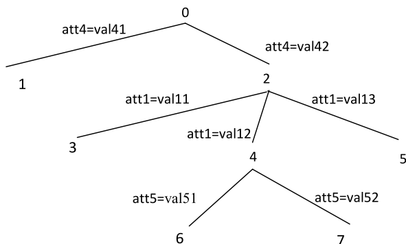
Figure 22.4 A Partly Developed CDH-Tree
