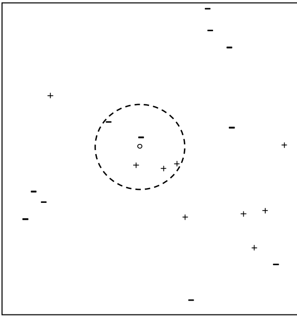
Figure 3.6 Two-dimensional Representation of Training Data in Figure 3.5
