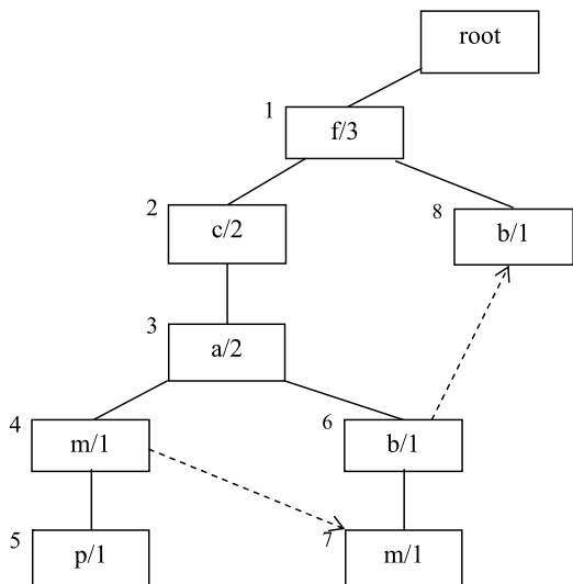
Figure 18.11 FP-tree After Processing All of Transaction 3
