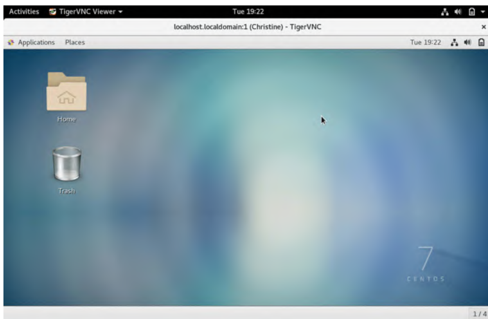
FIGURE 8.8 Using TigerVNC
