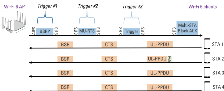
FIGURE 2-10: Uplink OFDMA.
