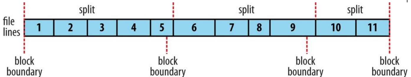
Figure 8-3. Logical records and HDFS blocks for TextInputFormat
