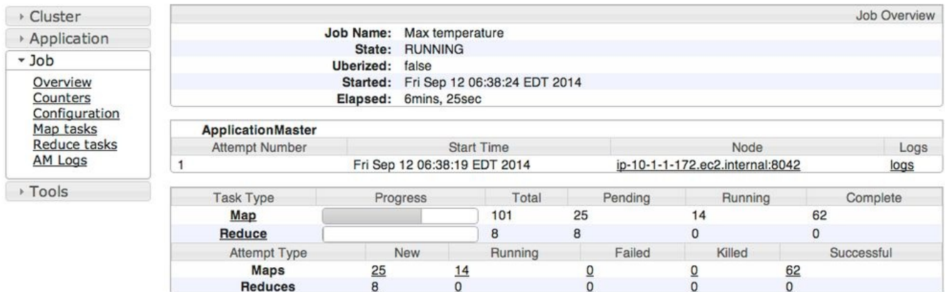
Figure 6-2. Screenshot of the job page
