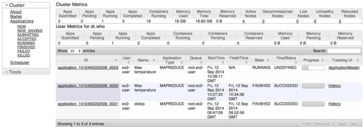
Figure 6-1. Screenshot of the resource manager page
