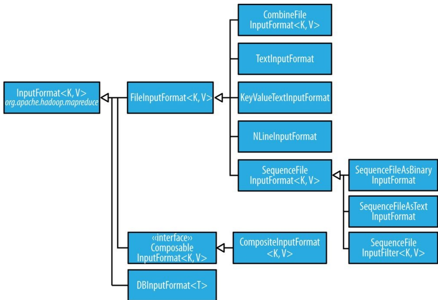
Figure 8-2. InputFormat class hierarchy
